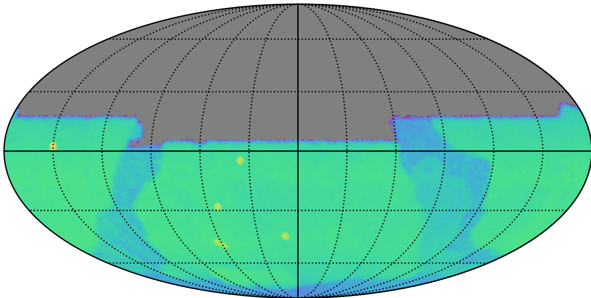
weather_cloudso14v3.5_10yrs u: CoaddM5
