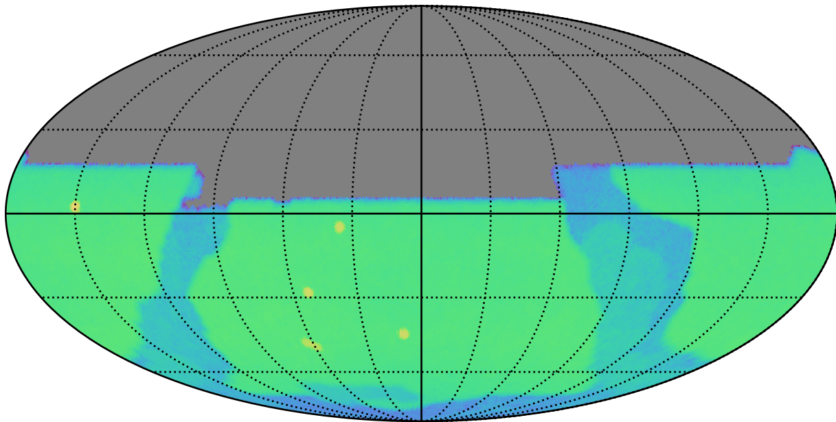
weather_cloudso14v3.5_10yrs y: CoaddM5
