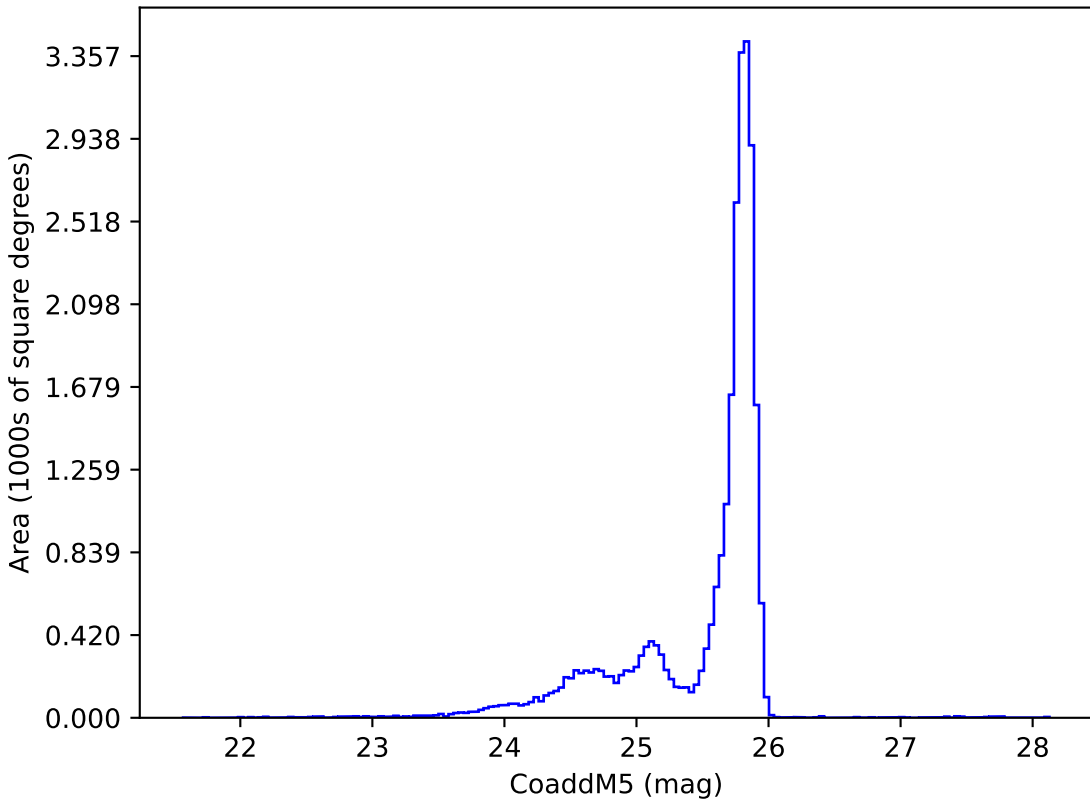
weather_cloudso14v3.5_10yrs z: CoaddM5
