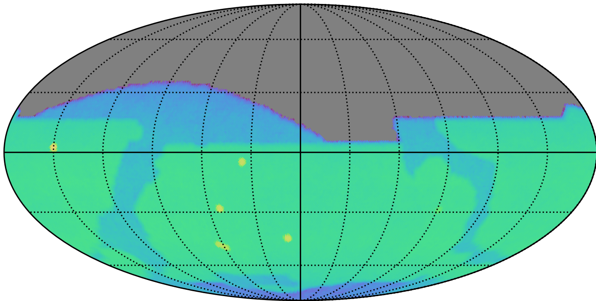
weather_cloudso14v3.5_10yrs z: CoaddM5
