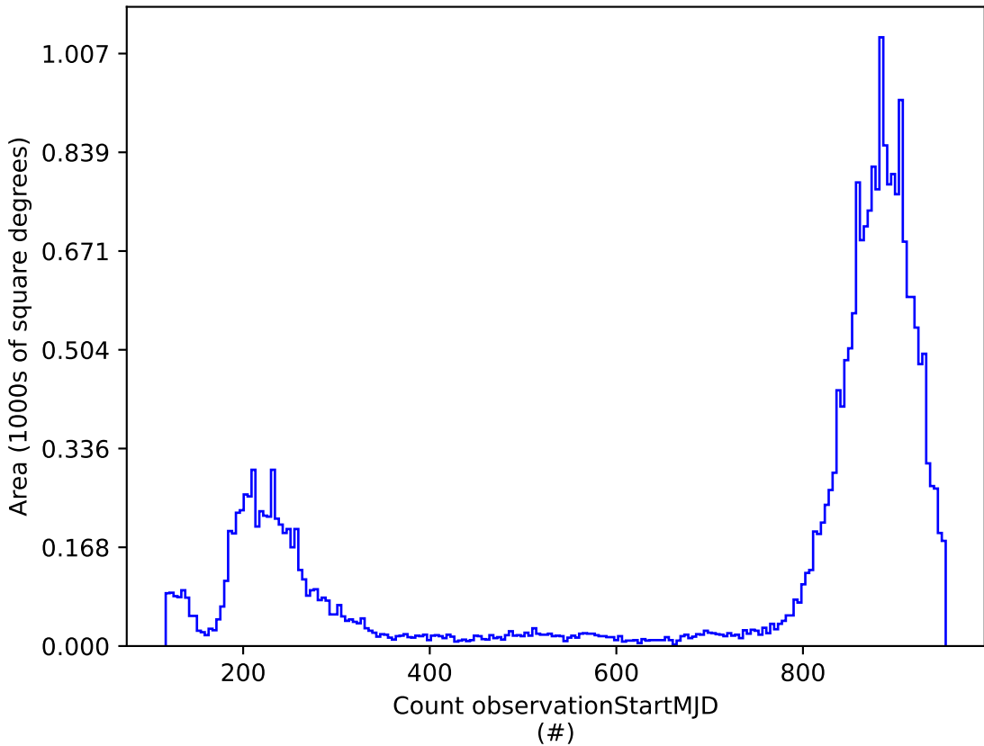
weather_cloudso14v3.5_10yrs : Count observationStartMJD
