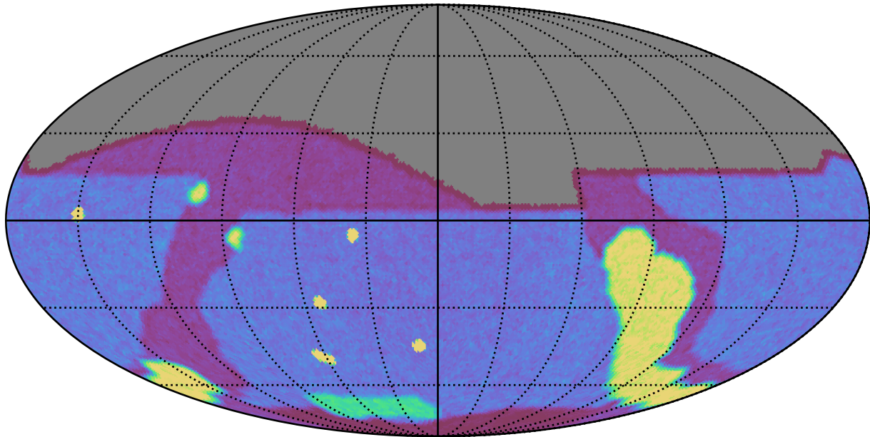
weather_cloudso14v3.5_10yrs g: Count observationStartMJD
