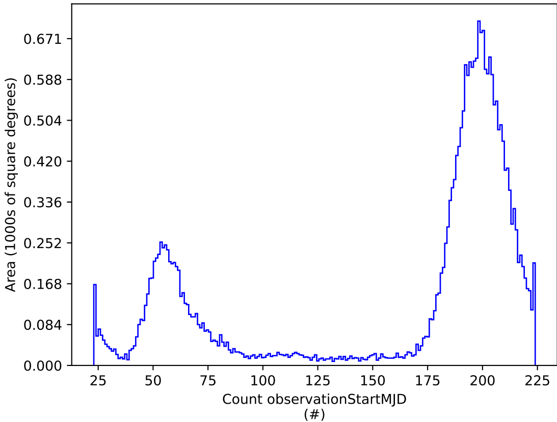
weather_cloudso14v3.5_10yrs i: Count observationStartMJD
