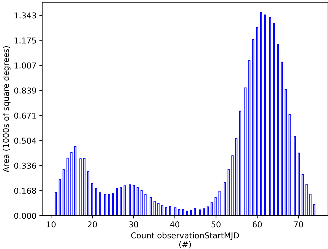
weather_cloudso14v3.5_10yrs u: Count observationStartMJD
