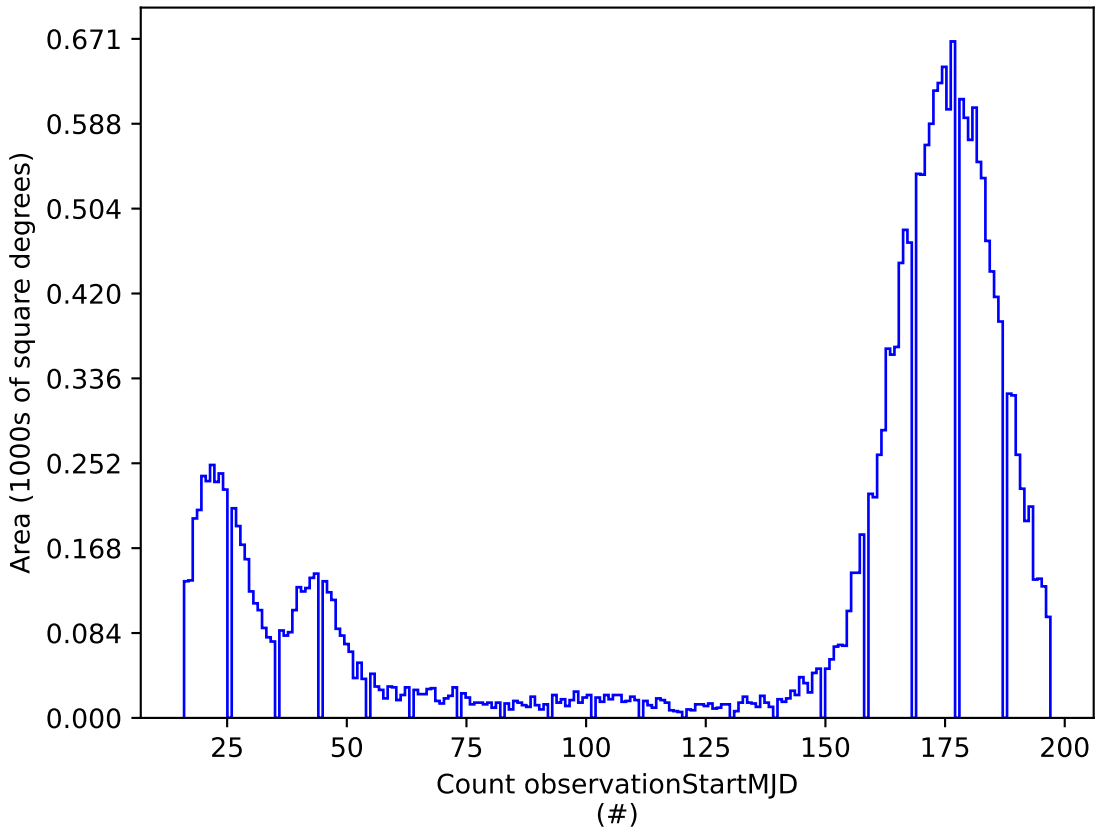
weather_cloudso14v3.5_10yrs y: Count observationStartMJD
