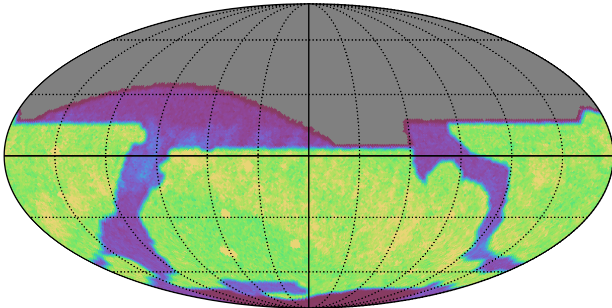
weather_cloudso14v3.5_10yrs z: Count observationStartMJD
