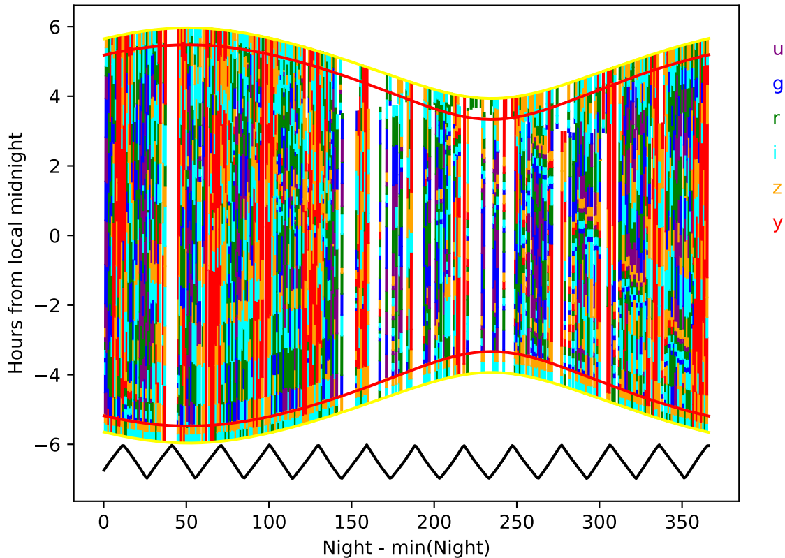
weather_cloudso14v3.5_10yrs year 0-1: Hourglass
