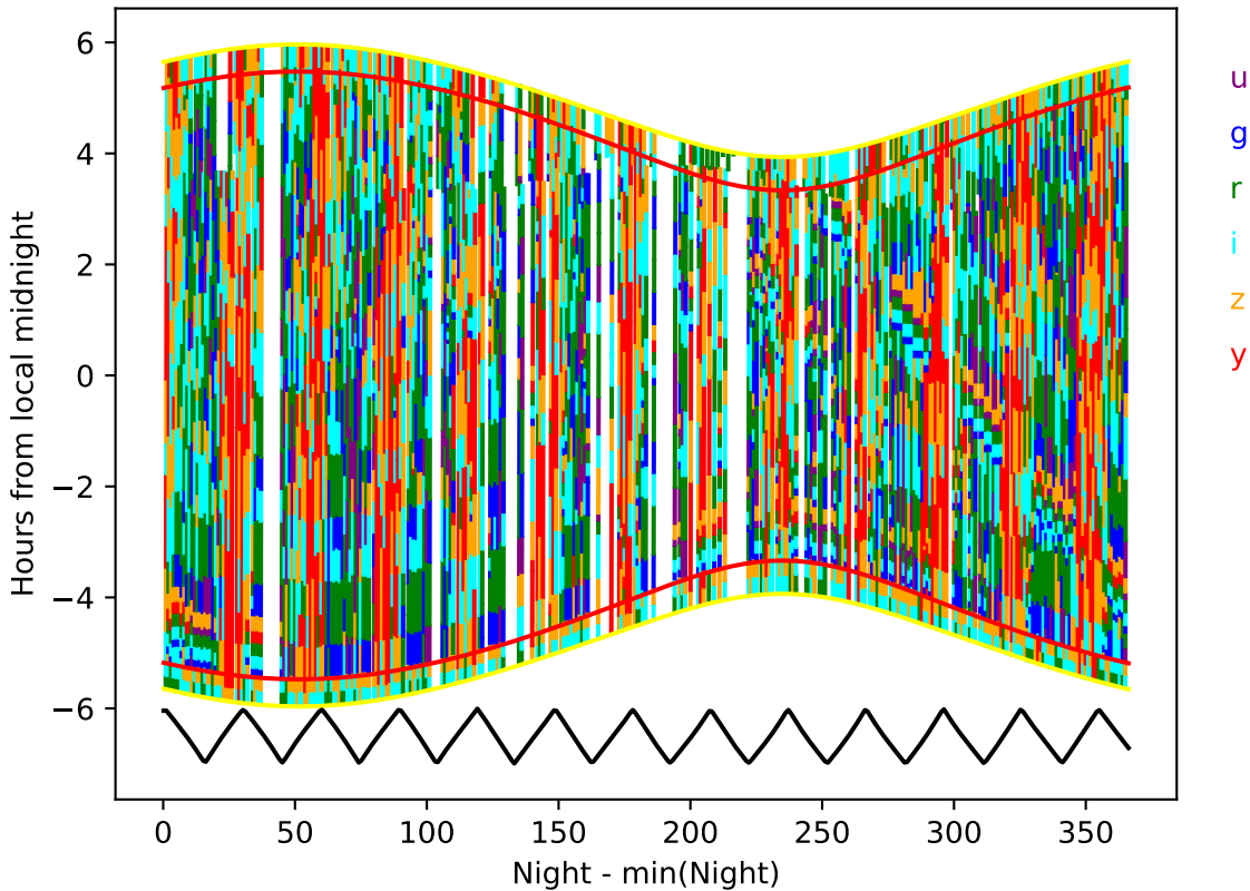
weather_cloudso14v3.5_10yrs year 1-2: Hourglass
