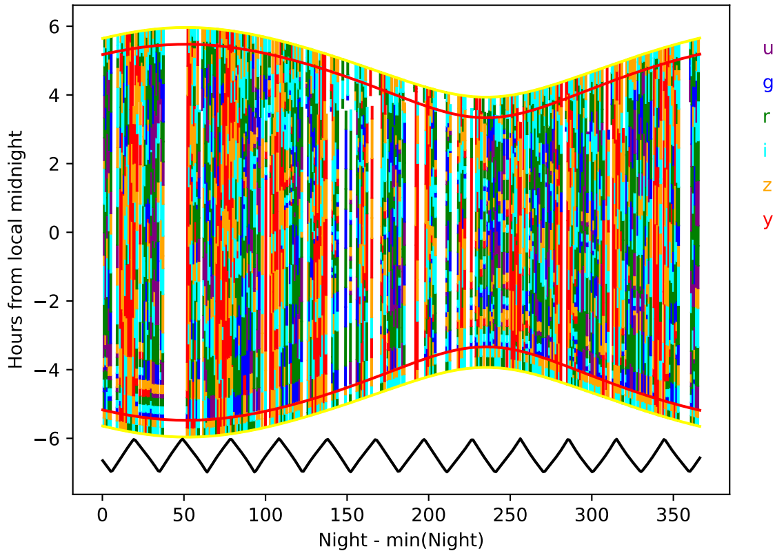
weather_cloudso14v3.5_10yrs year 2-3: Hourglass
