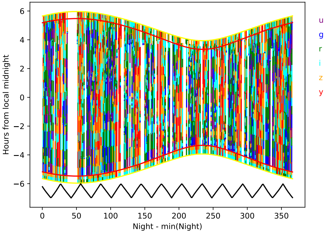
weather_cloudso14v3.5_10yrs year 4-5: Hourglass
