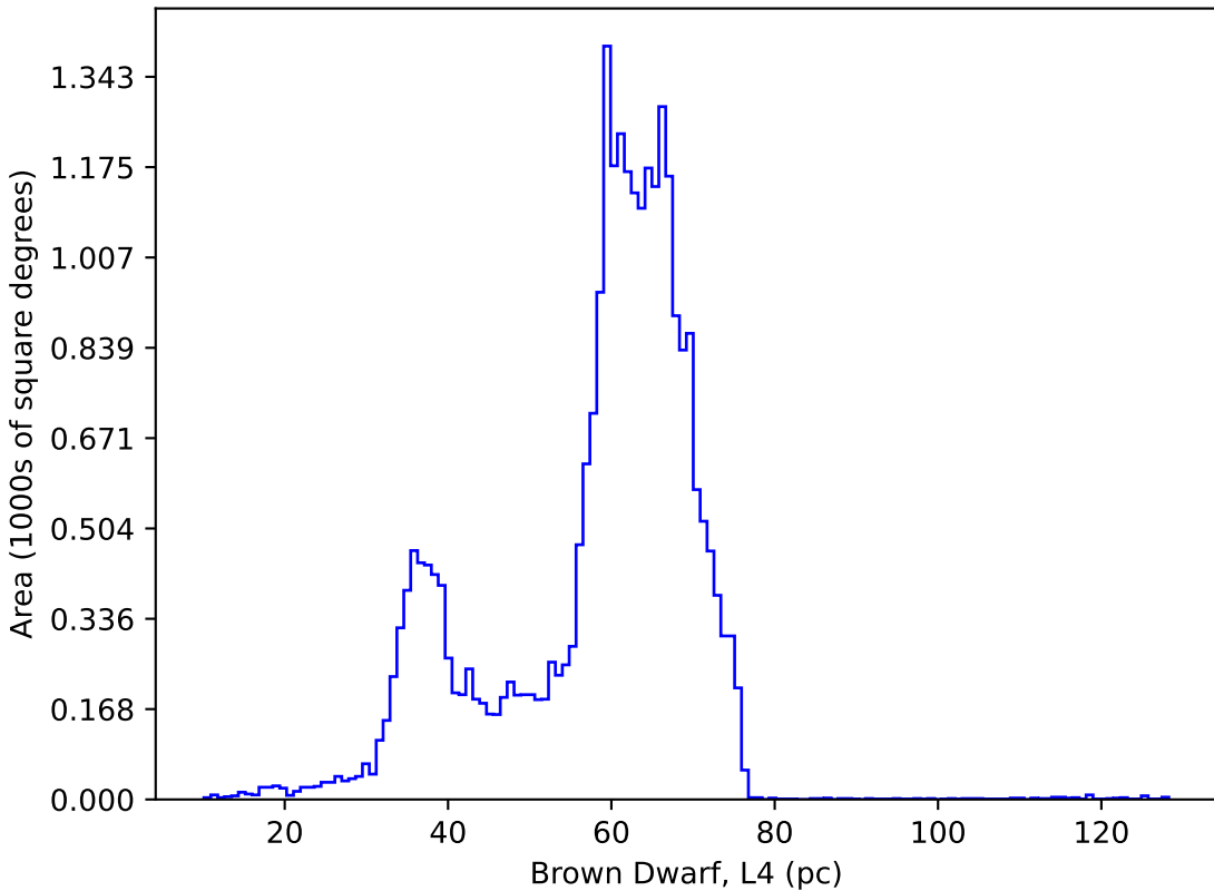
weather_cloudso14v3.5_10yrs : Brown Dwarf, L4
