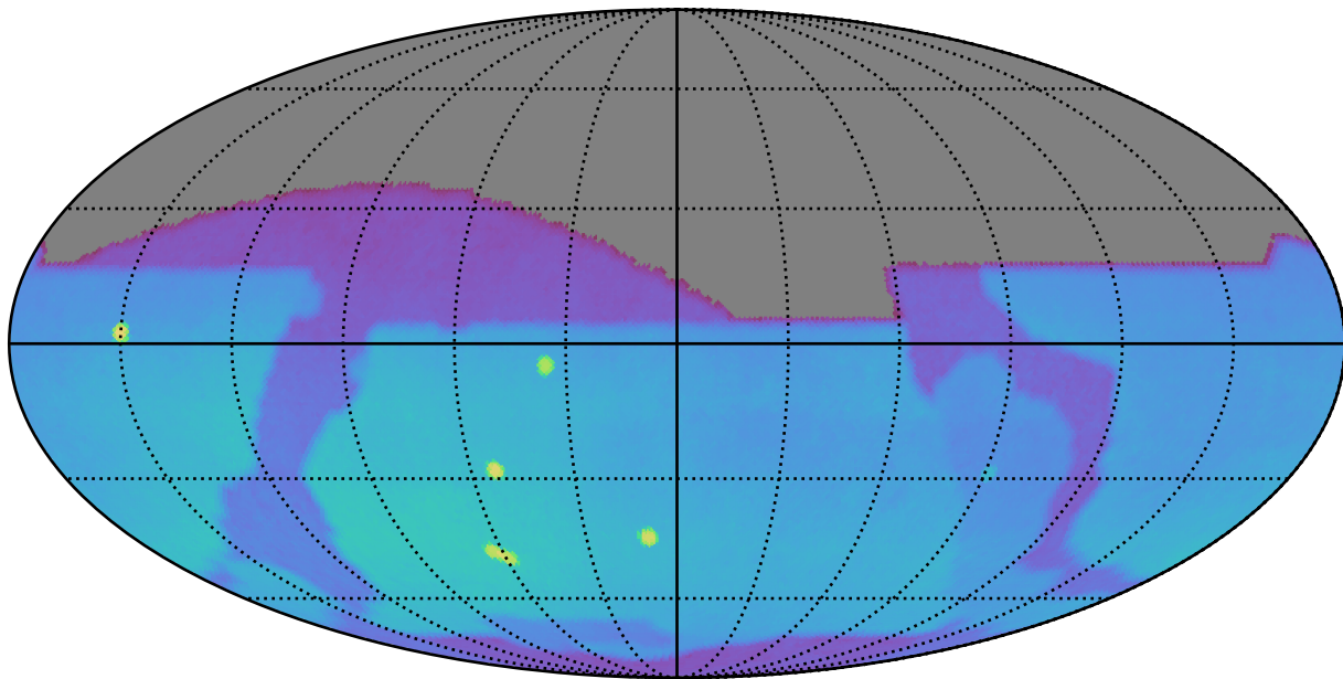
weather_cloudso14v3.5_10yrs : Brown Dwarf, L4
