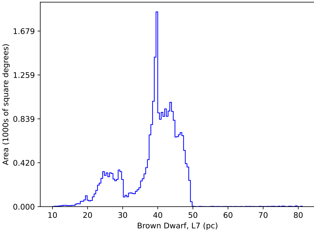
weather_cloudso14v3.5_10yrs : Brown Dwarf, L7
