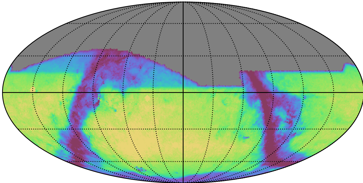
weather_cloudso14v3.5_10yrs r: GalaxyCountsMetricExtended
