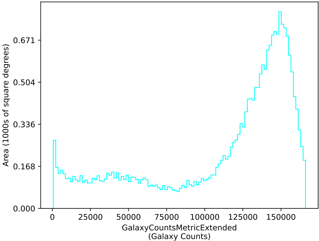
weather_cloudso14v3.5_10yrs u: GalaxyCountsMetricExtended
