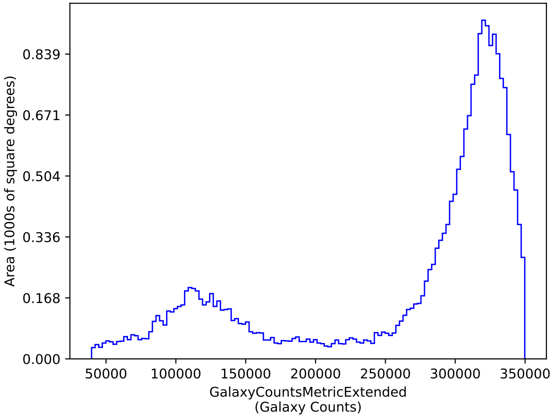
weather_cloudso14v3.5_10yrs y: GalaxyCountsMetricExtended
