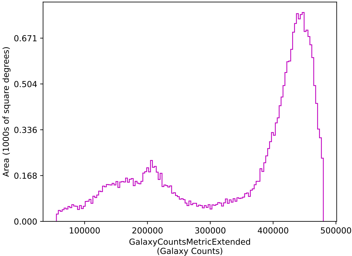
weather_cloudso14v3.5_10yrs z: GalaxyCountsMetricExtended
