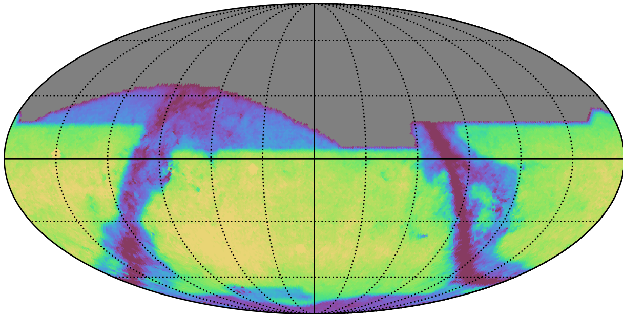
weather_cloudso14v3.5_10yrs z: GalaxyCountsMetricExtended
