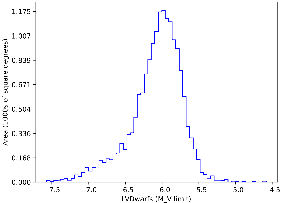
weather_cloudso14v3.5_10yrs gi: LVDwarfs
