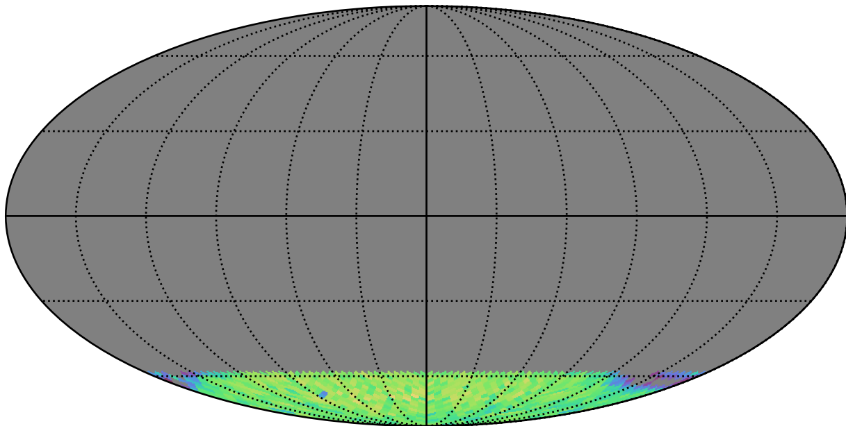
weather_cloudso14v3.5_10yrs gi SCP: LVDwarfs
