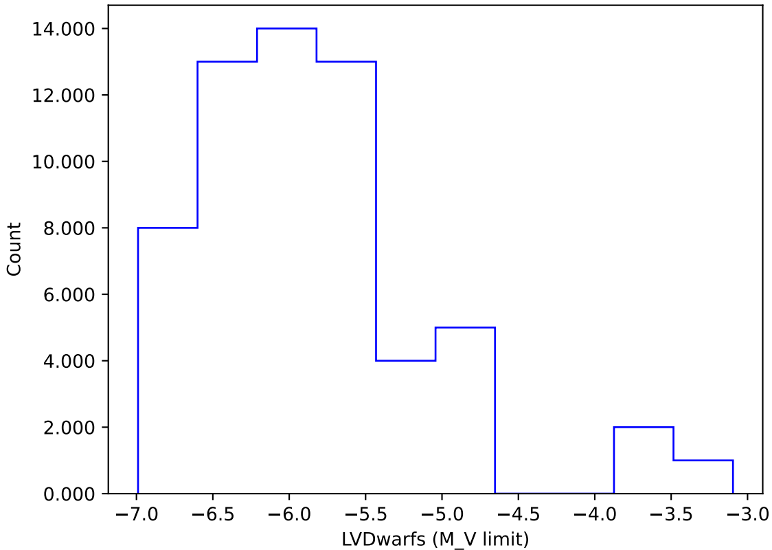
weather_cloudso14v3.5_10yrs gi: LVDwarfs
