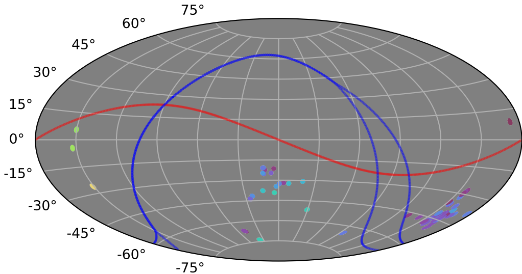
weather_cloudso14v3.5_10yrs gi: LVDwarfs
