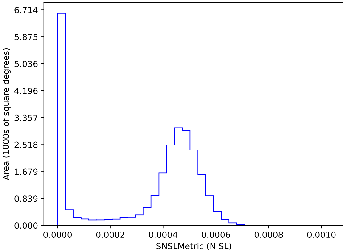
weather_cloudso14v3.5_10yrs : SNSLMetric
