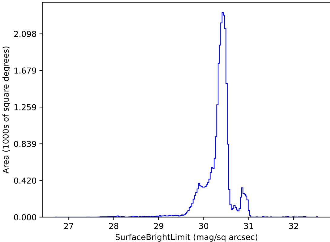
weather_cloudso14v3.5_10yrs g: SurfaceBrightLimit
