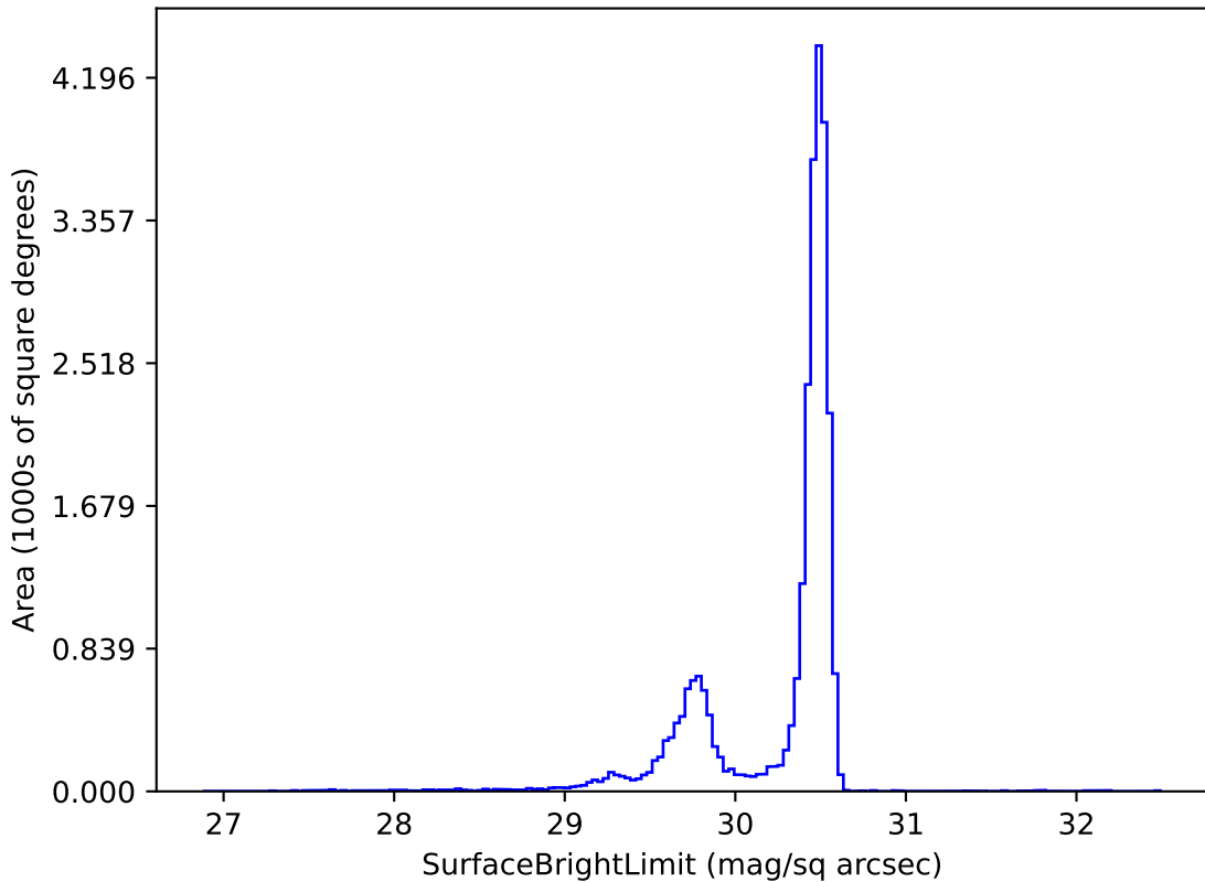
weather_cloudso14v3.5_10yrs r: SurfaceBrightLimit
