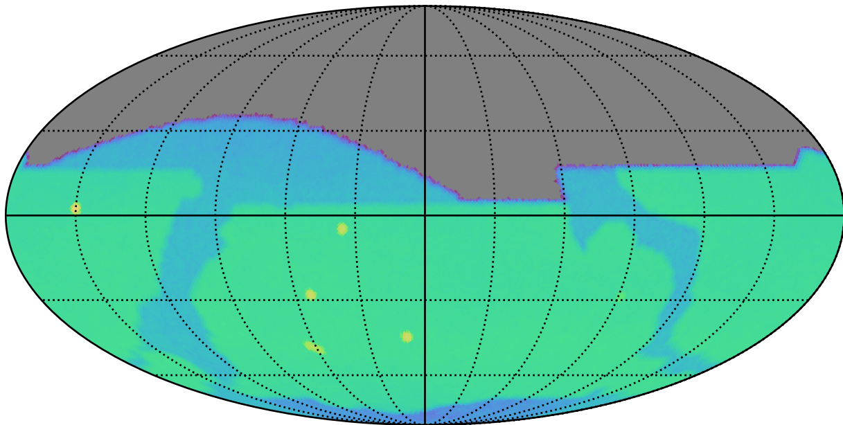
weather_cloudso14v3.5_10yrs r: SurfaceBrightLimit
