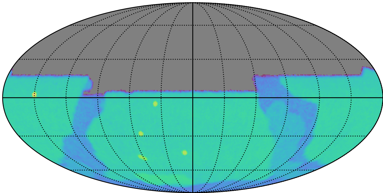
weather_cloudso14v3.5_10yrs u: SurfaceBrightLimit
