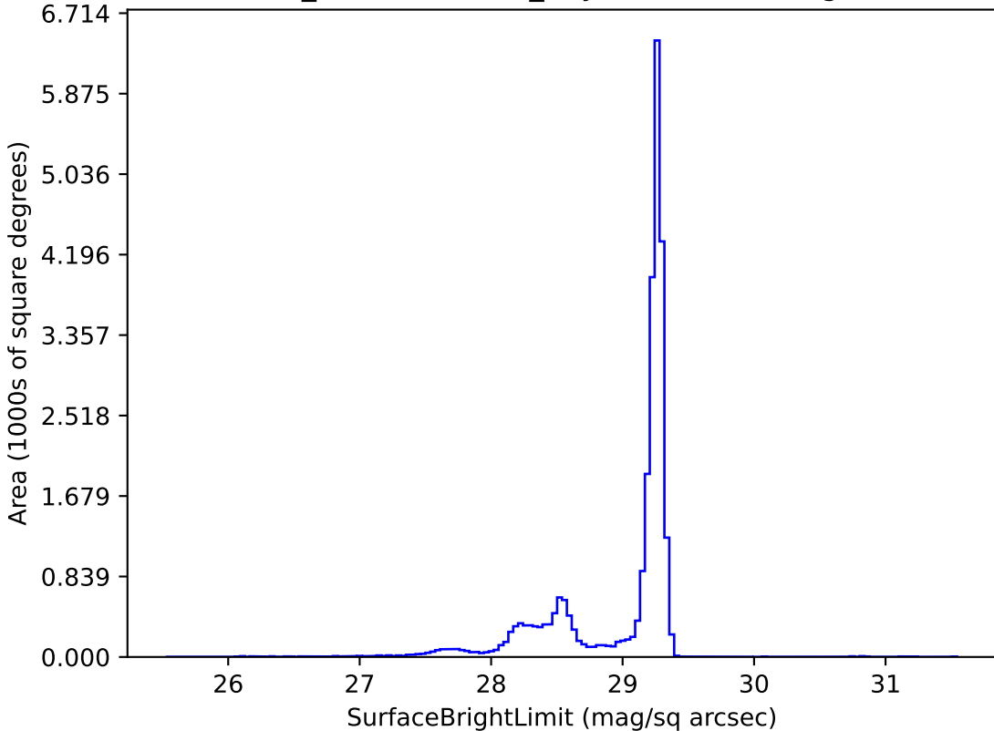
weather_cloudso14v3.5_10yrs z: SurfaceBrightLimit
