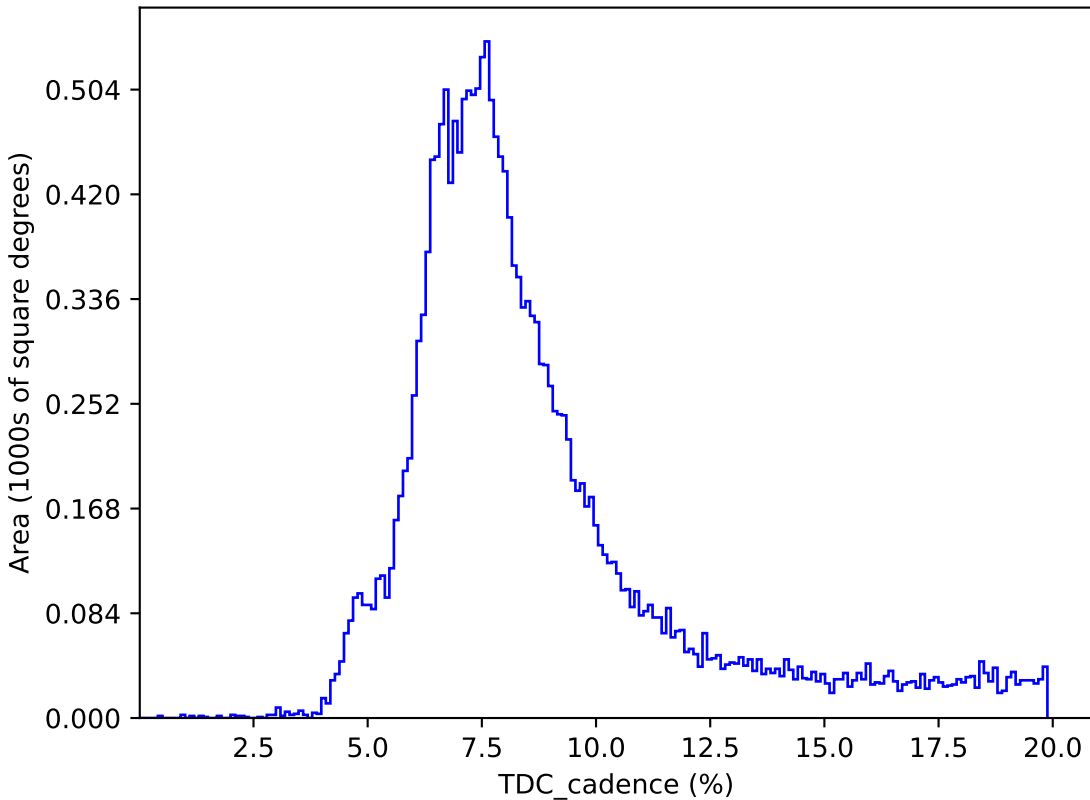
weather_cloudso14v3.5_10yrs : TDC_cadence
