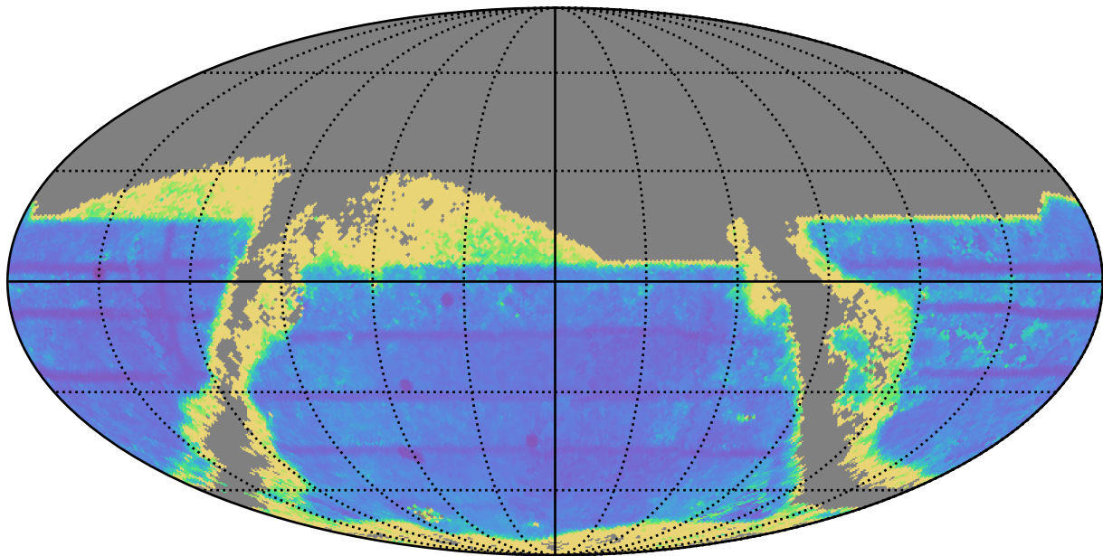
weather_cloudso14v3.5_10yrs : TDC_precision
