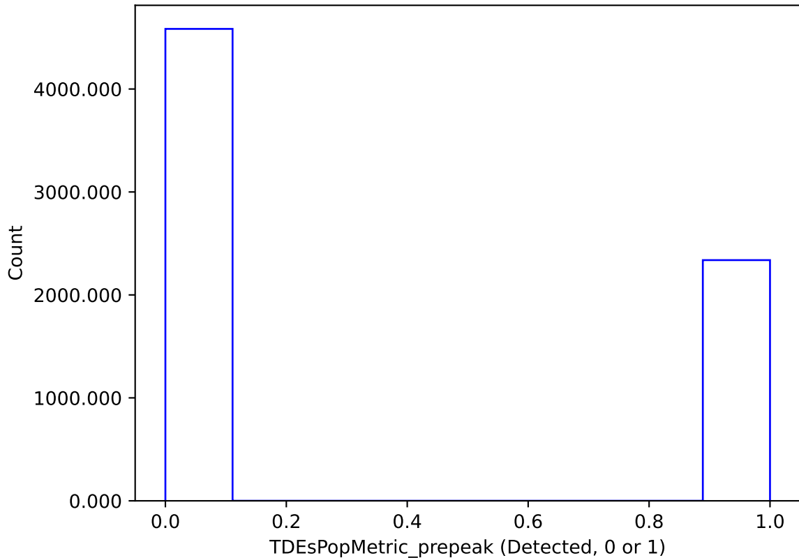
weather_cloudso14v3.5_10yrs : TDEsPopMetric_prepeak
