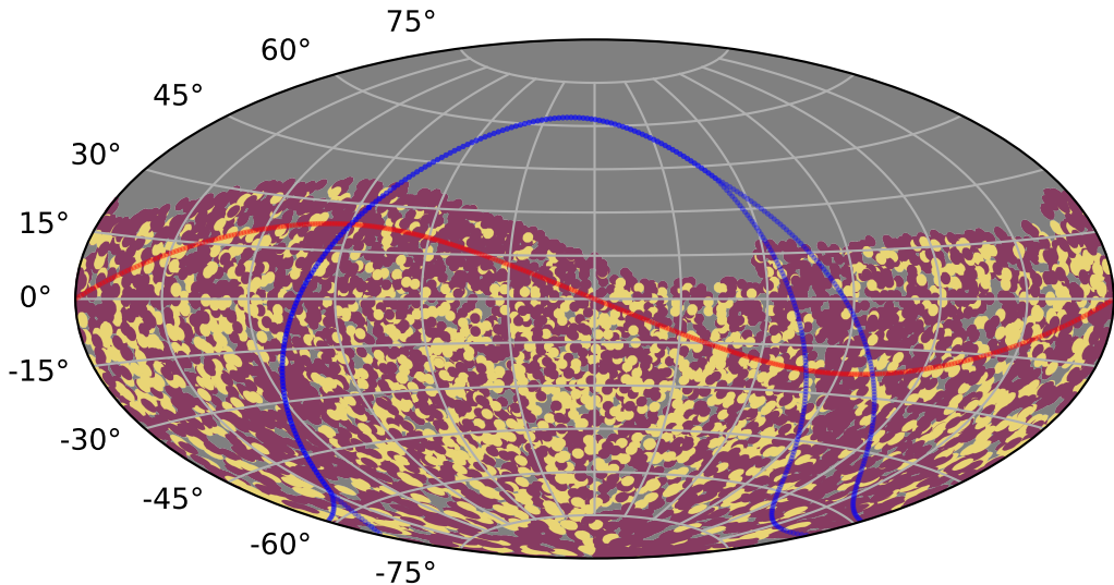
weather_cloudso14v3.5_10yrs : TDEsPopMetric_prepeak
