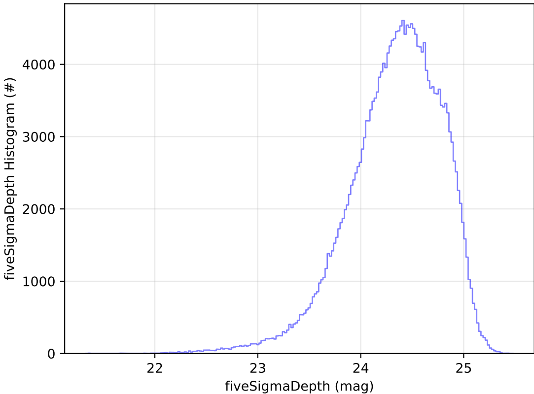
weather_cloudso14v3.5_10yrs g: fiveSigmaDepth Histogram
