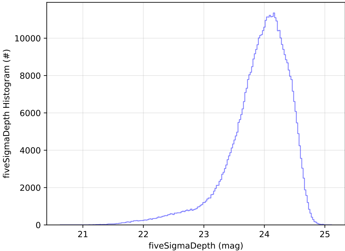
weather_cloudso14v3.5_10yrs r: fiveSigmaDepth Histogram
