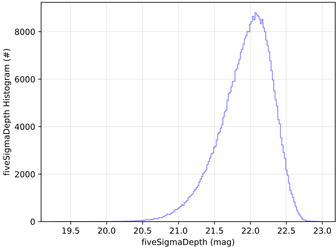
weather_cloudso14v3.5_10yrs y: fiveSigmaDepth Histogram
