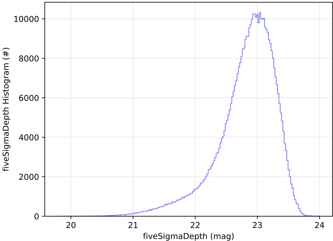
weather_cloudso14v3.5_10yrs z: fiveSigmaDepth Histogram
