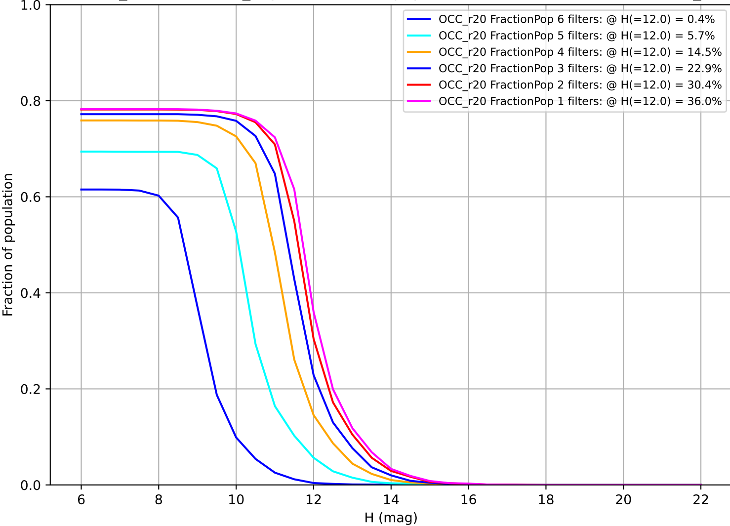
weather_cloudso14v3.5_10yrs: Fraction of population with colors in X filters OCC_r20
