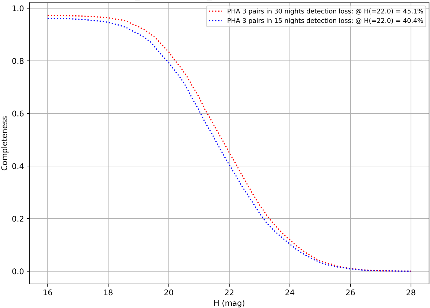
weather_cloudso14v3.5_10yrs: DifferentialCompleteness
