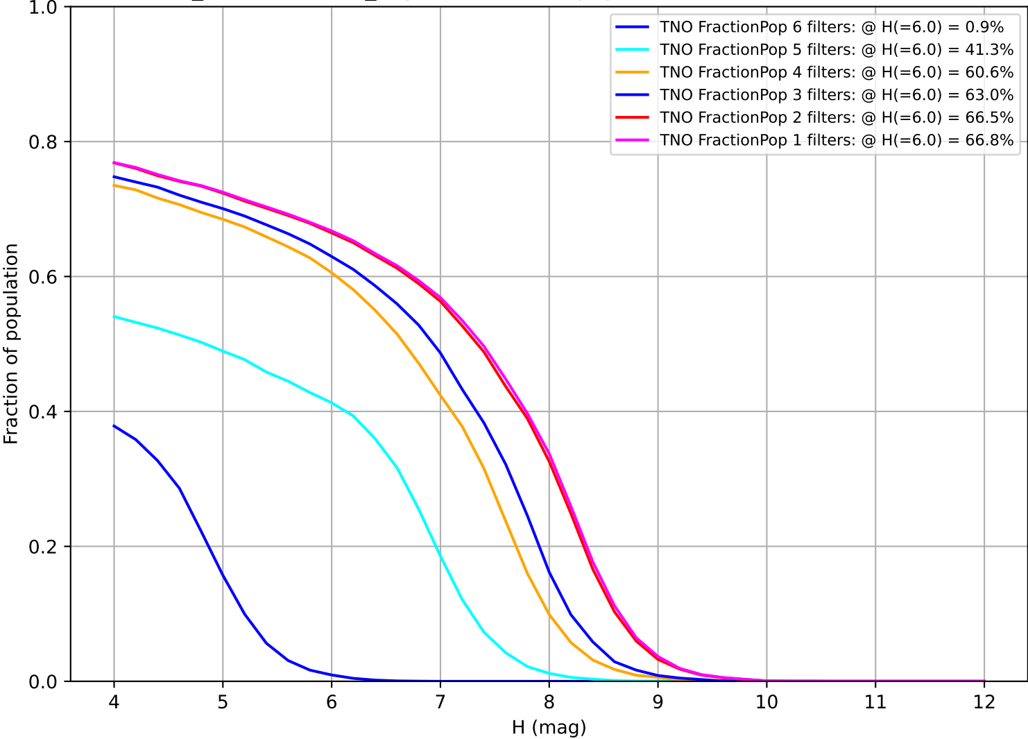
weather_cloudso14v3.5_10yrs: Fraction of population with colors in X filters TNO
