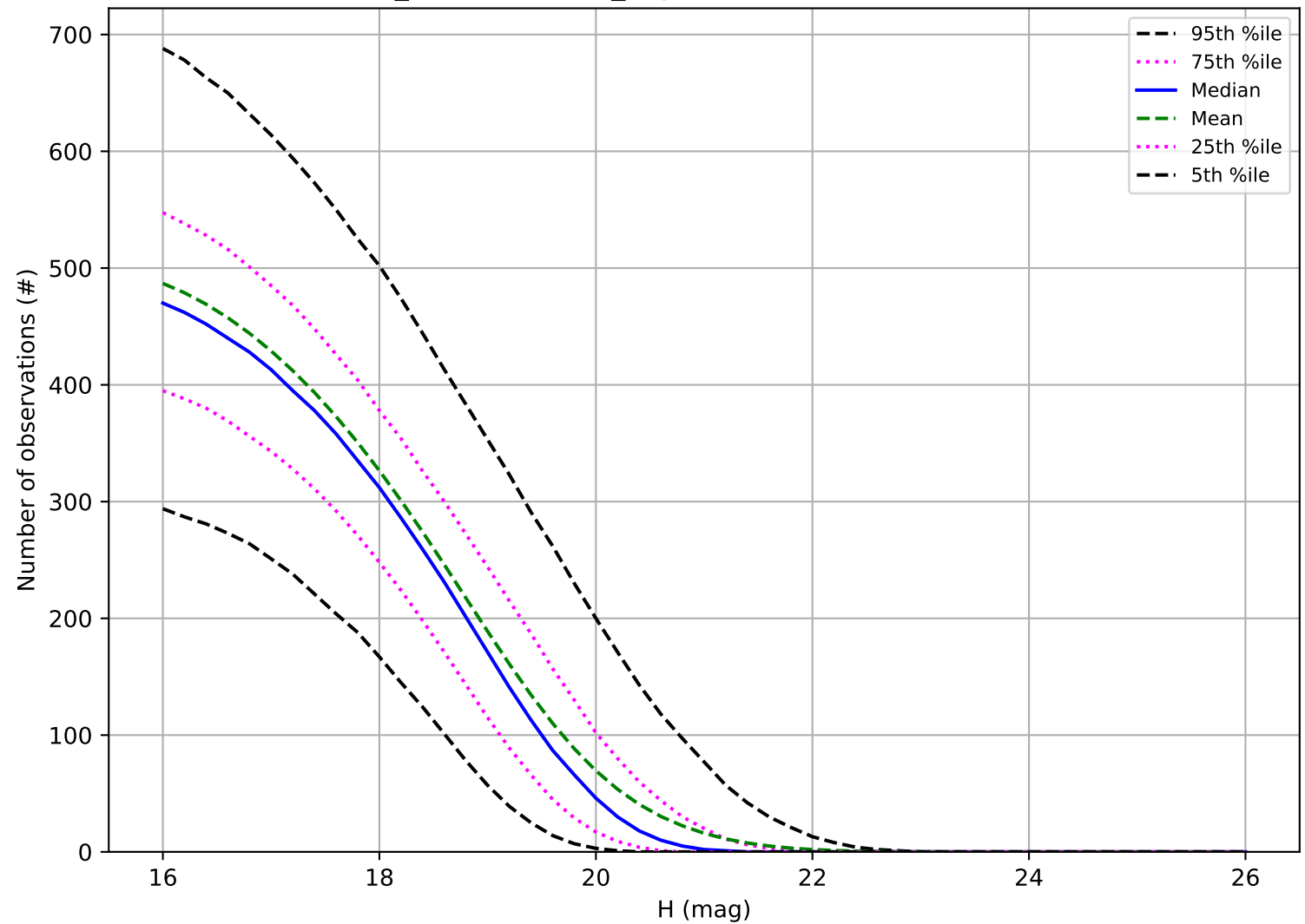
weather_cloudso14v3.5_10yrs: Number of observations MBA
