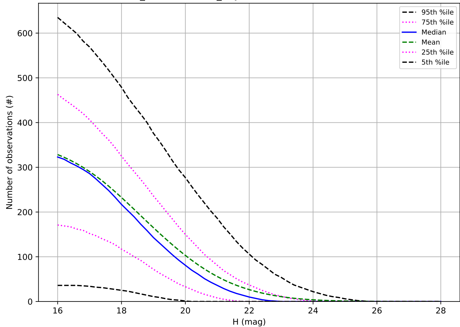
weather_cloudso14v3.5_10yrs: Number of observations NEO
