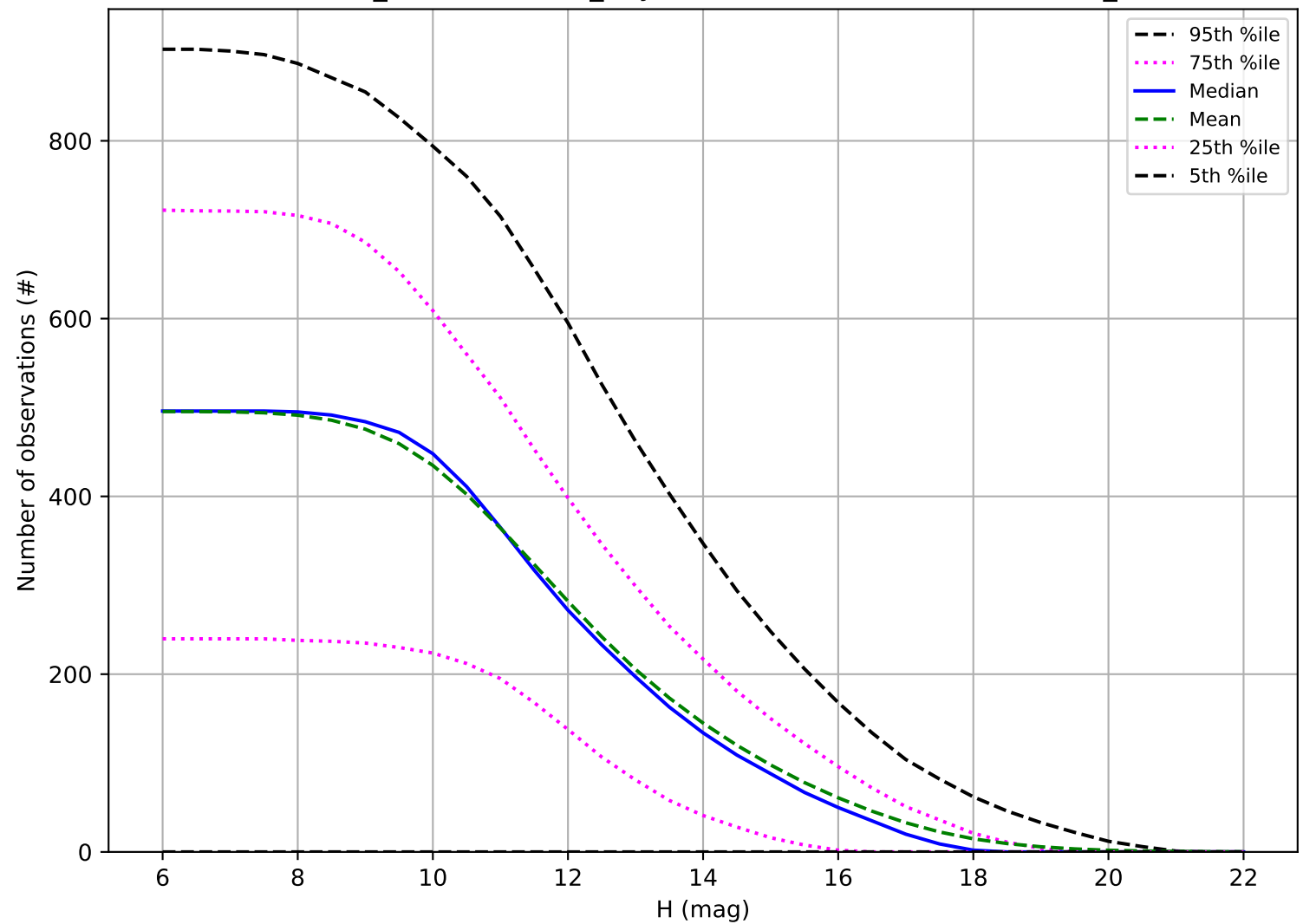
weather_cloudso14v3.5_10yrs: Number of observations OCC_r5
