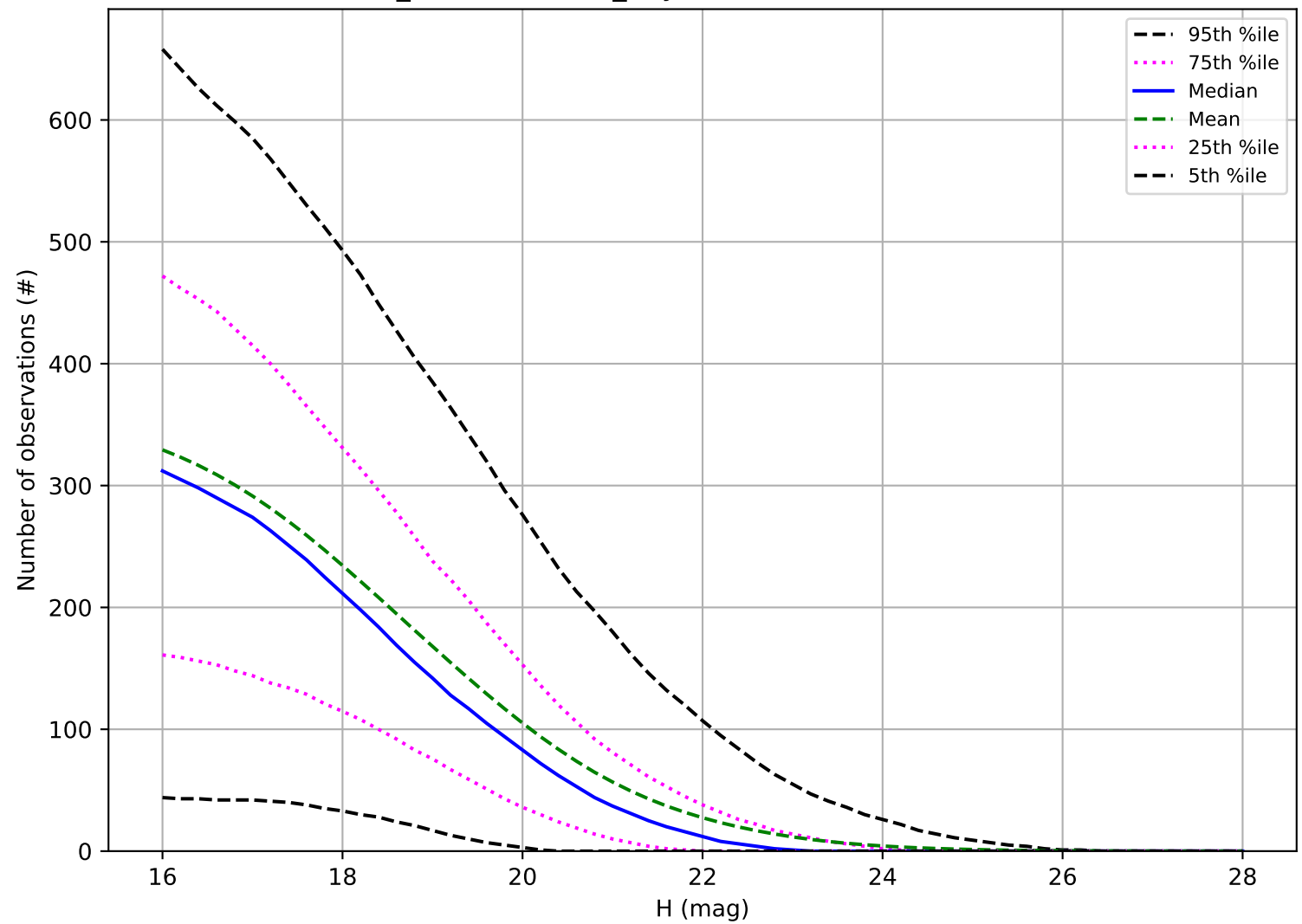
weather_cloudso14v3.5_10yrs: Number of observations PHA
