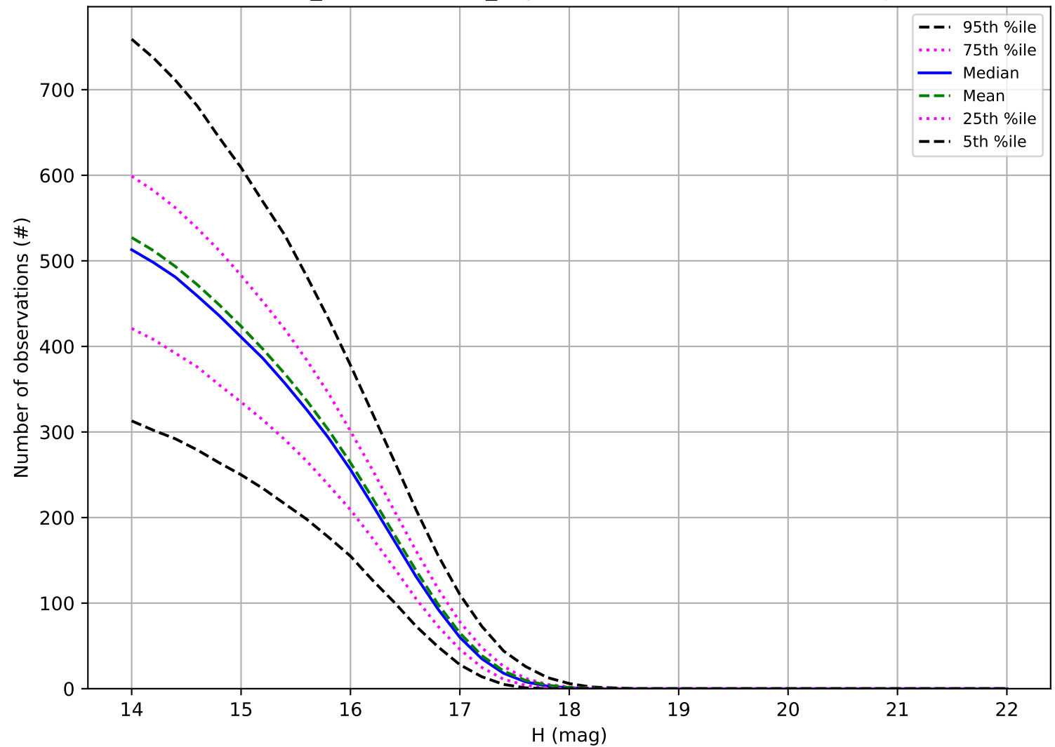
weather_cloudso14v3.5_10yrs: Number of observations Trojan
