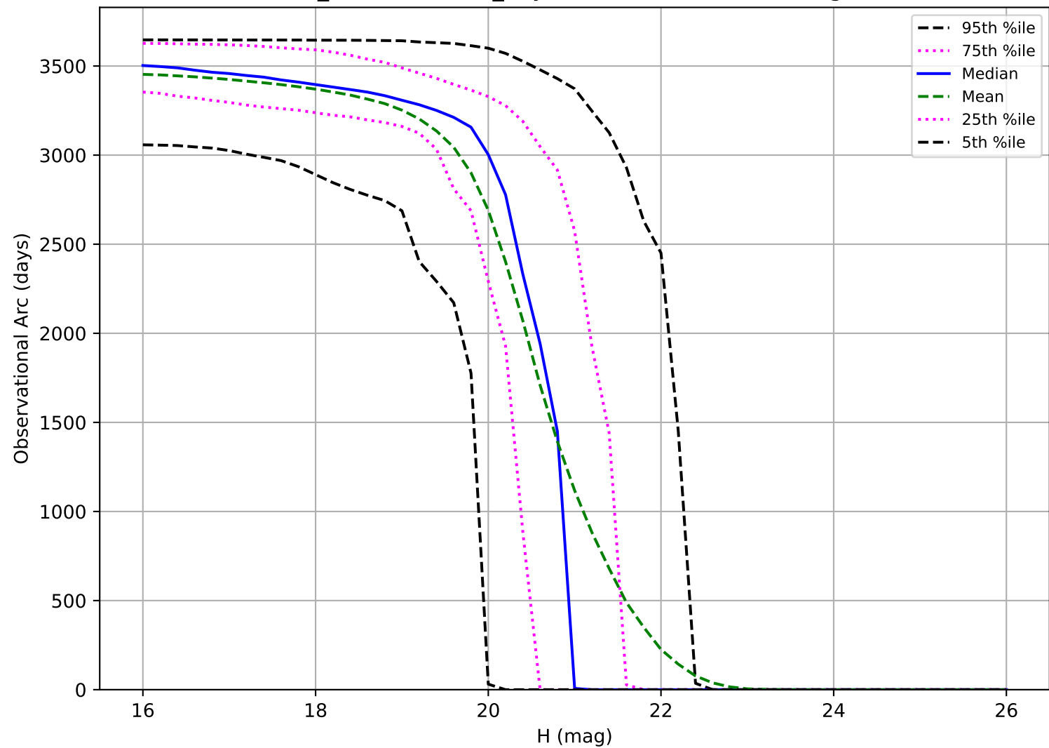
weather_cloudso14v3.5_10yrs: Observational Arc Length MBA
