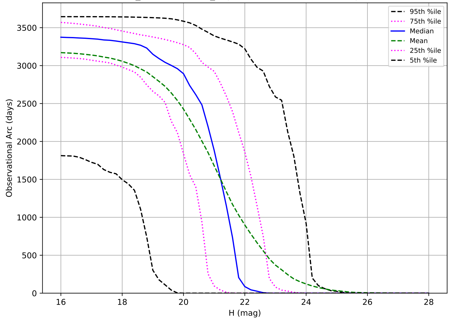
weather_cloudso14v3.5_10yrs: Observational Arc Length NEO
